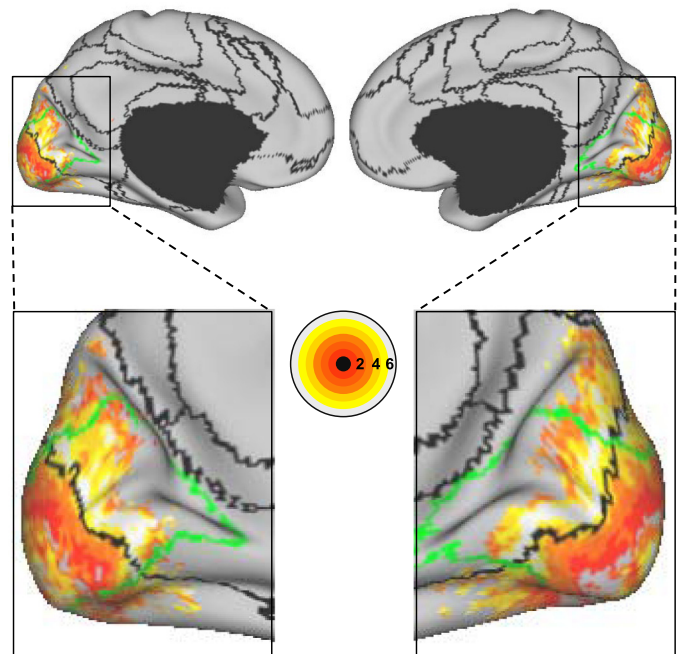
Fig. 15. Eccentricity estimates quantify the division of the early visual cortex into central and peripheral systems. Eccentricity estimates in the early visual areas of 4 subjects were averaged and overlaid on the boundaries (in black) of the 17-network estimate. The boundary between areas 18 and 19 estimated from the histological data set is overlaid in green. The 17-network estimate divides the early visual areas along an isoeccentricity line of \sim 4^\circ . Note that the eccentricity estimates are not reliable outside the V1-V3 complex.
