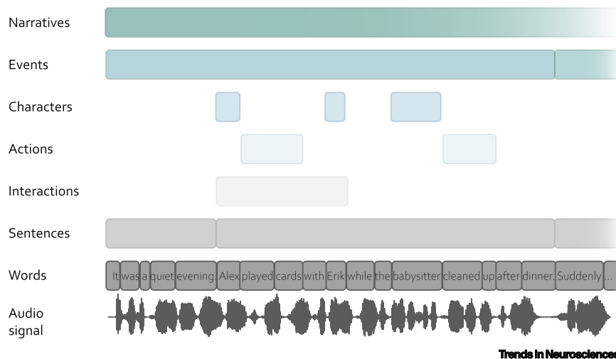
Figure 1. Narratives Comprise Many Layers of Nested Features. These features can for instance include (from bottom to top in the schematic): phonemes, words, sentences, social interactions, actions, characters, events, and narrative context. As such, narrative stimuli allow researchers to study a variety of cognitive and perceptual processes. Gradually emerging narrative context can modulate processing of individual embedded features; this kind of contextual modulation is absent from more traditional paradigms comprising strictly controlled and decontextualized stimuli. By leveraging narrative stimuli and computational models, neural mechanisms underlying cognitive processes for each feature of interest can be isolated during naturalistic experience. This approach can allow researchers to take a step toward generalizing their findings beyond the laboratory setting and can advance our understanding of how different cognitive processes interact during real-world experience.
